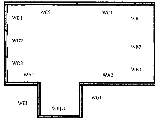
Fig. 4. Wall panel layout for SIP home
