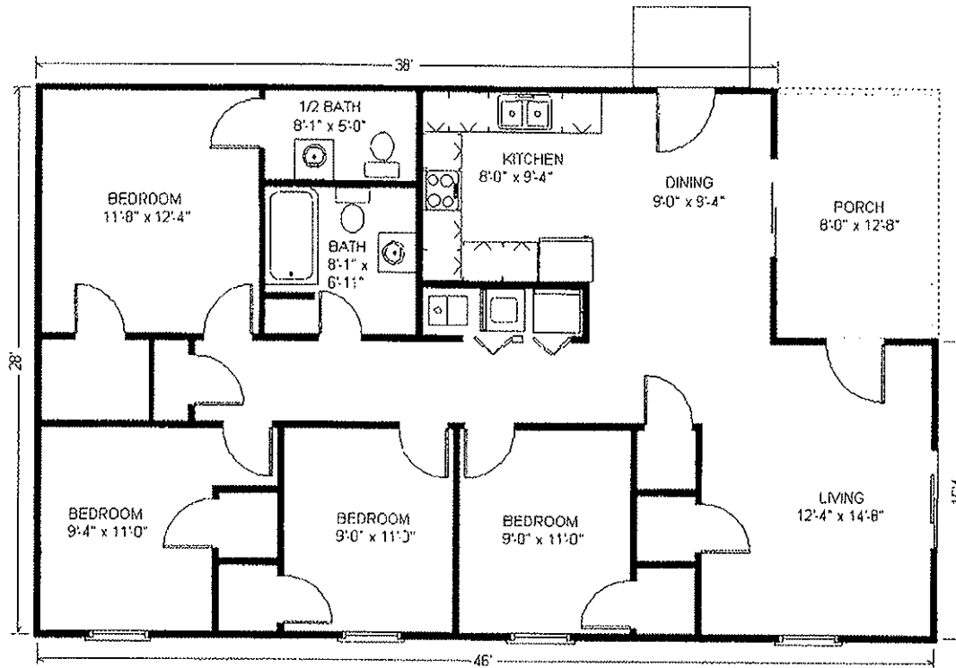
Fig. 3. Floor plan for conventional wood-framed home
