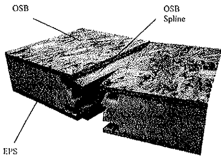
Fig. 1. Typical structural insulated panel configuration
