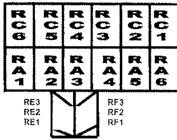
Fig. 5. Roof panel layout for SIP home
