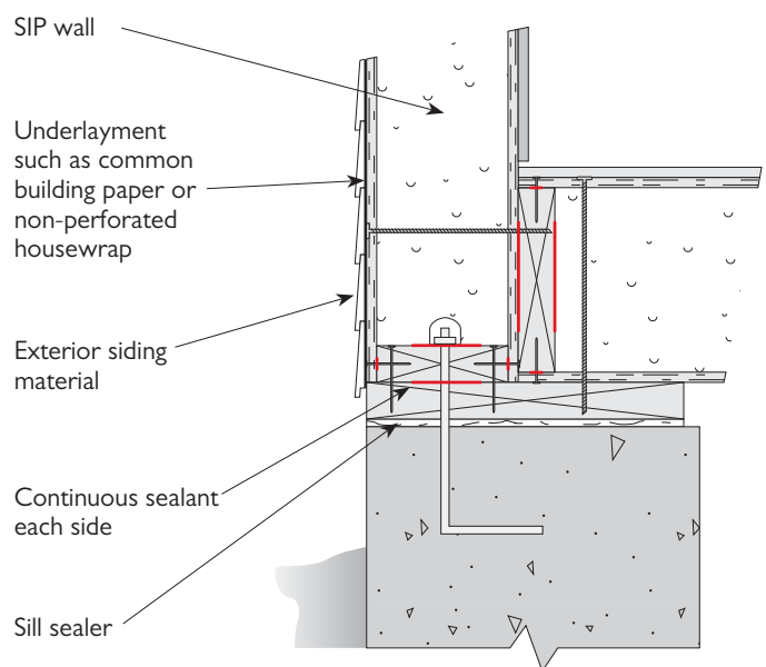
FIGURE 2 — Foundation Framing
