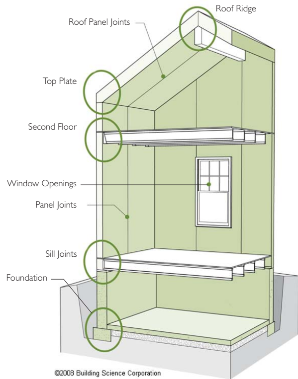
FIGURE 1 — Take special note of the connection details and installation instructions for these areas. Contact your SIPA member manufacturer for complete detail drawings, technical specifications and installation instructions. You can also access many of these documents from our website at www.sips.org .
