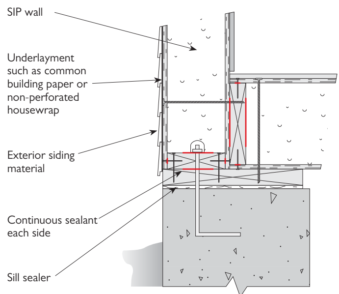
FIGURE 2 — Foundation Framing
